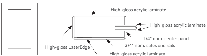
Shaker profile
